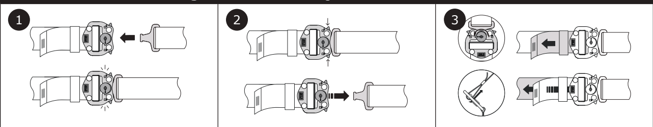
Figure 8B - Duo-Lok Quick Connect Buckles
