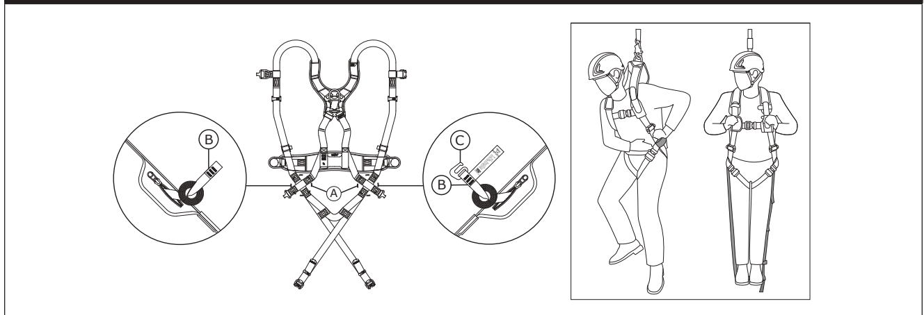
Figure 12 - Activation des sangles anti-traumatisme
