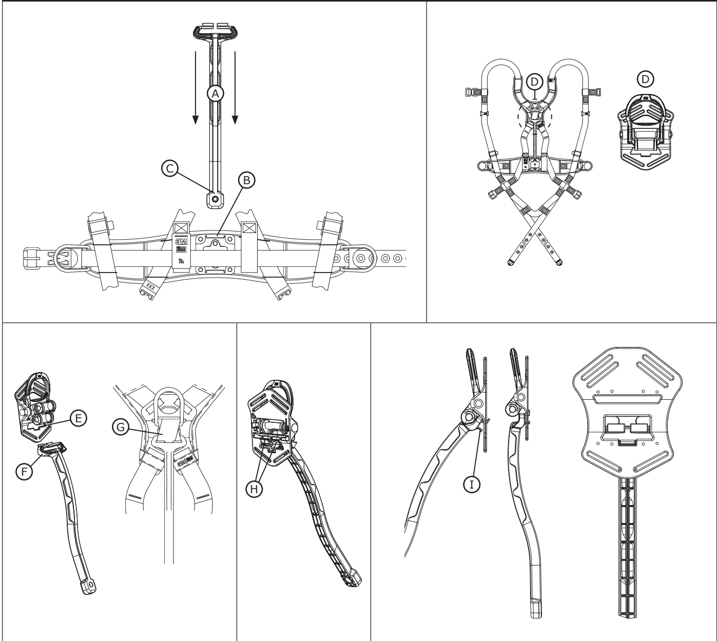
Figure 11 - Attaching the Weight Distribution System
