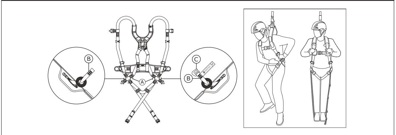
Figure 12 - Activating the Trauma Straps
