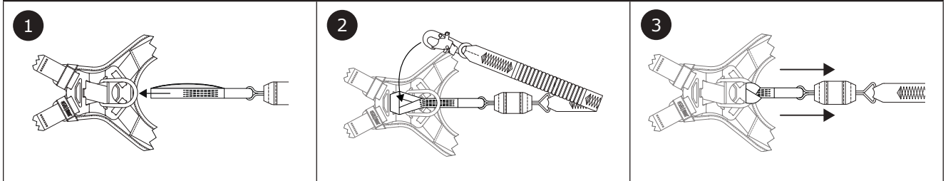
Figure 13 - Securing Lanyards with Choker Loops
